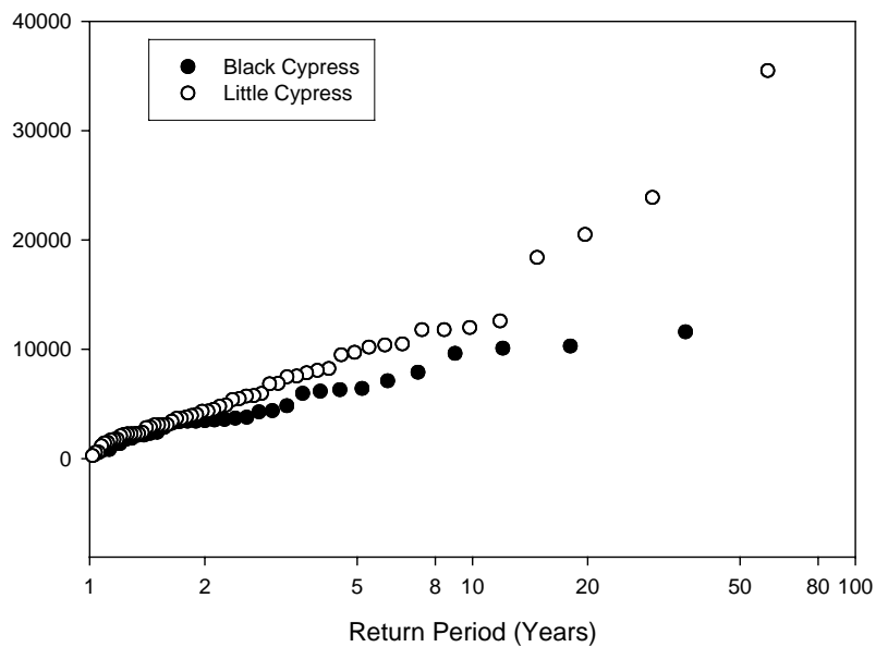
Figure 6. Flow recurrence for Black Cypress Bayou and Little Cypress Creek at Jefferson.
