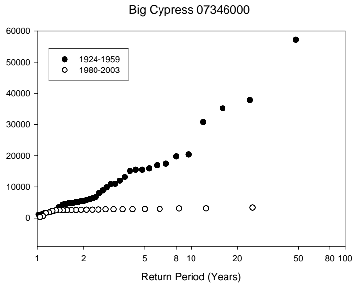
Figure 5. Flow recurrence graph for Big Cypress Creek at Jefferson for pre and post-dam years
