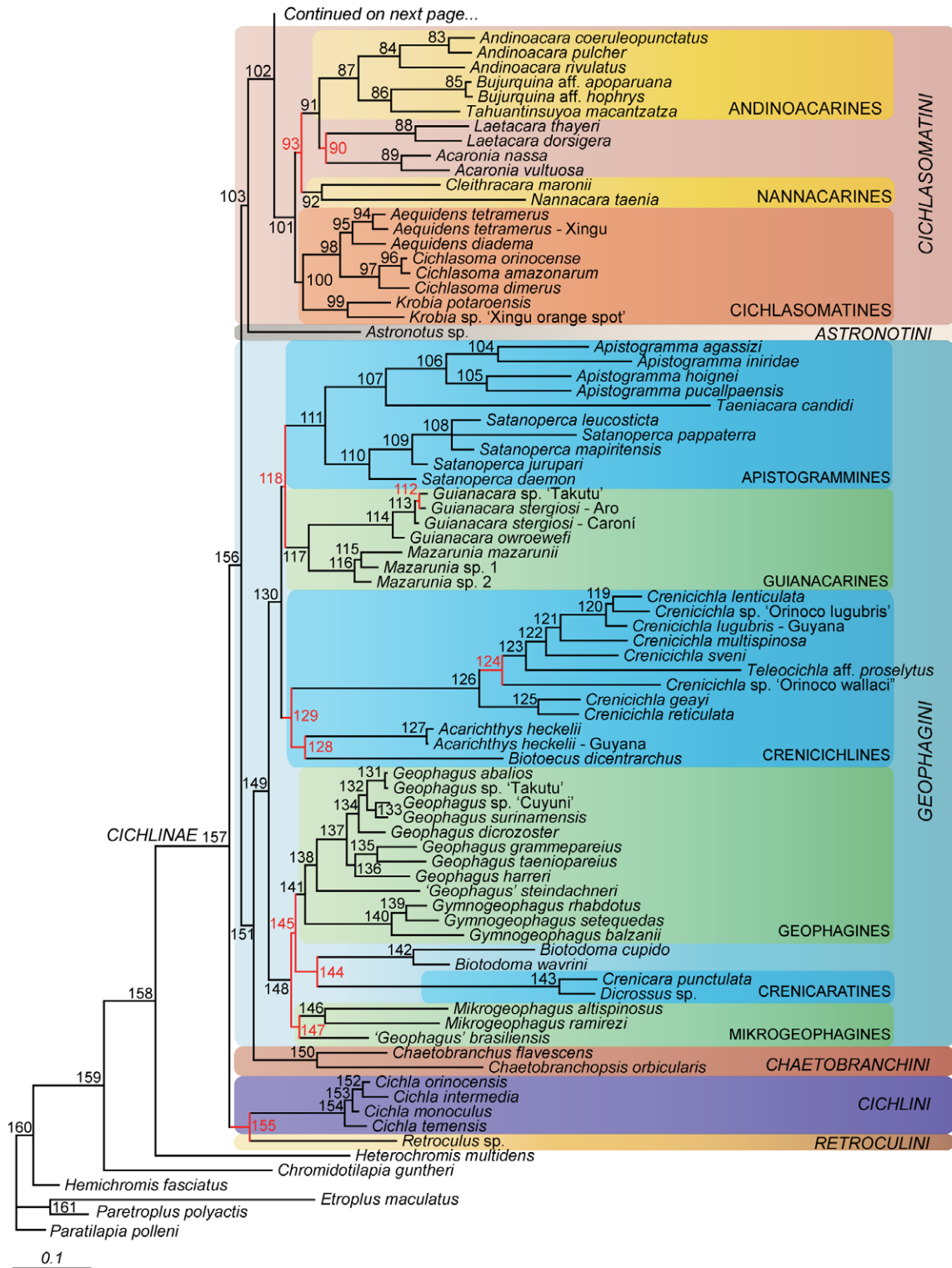
Fig. 1. Phylogenetic relationships of Neotropical cichlid fishes proposed in this paper based on 3868 base pairs from five loci. The tree represents Bayesian relationships recovered in a partitioned, unlinked analysis with 12 \times 10^6 replications using three mitochondrial (16S, Cytochrome b , ND4) and two nuclear DNA fragments (S7 Intron 1, RAG2). Node numbers correspond to those given in Table 2 providing support for the topology under Bayesian, Maximum Likelihood and Maximum Parsimony optimality criteria. Red numbers and branches depict branches whose length is not statistically different from zero according to the Internal Branch Test (see Section 2). Taxa accompanied by an asterisk have South American distribution but show phylogenetic affinity with the Central American Heroini. Colored boxes illustrate the composition of each clade as per the nomenclature used throughout the paper. (For interpretation of the references to color in this figure legend, the reader is referred to the web version of this article.)
